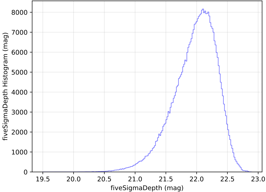
too_elab_heavy_r128_d2_gz_v3.4_10yrs All sky y band: fiveSigmaDepth Histogram
