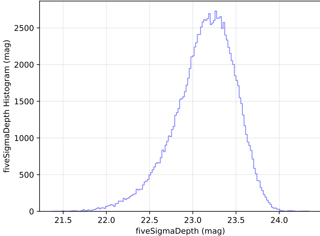
too_elab_heavy_r128_d2_gz_v3.4_10yrs All sky u band: fiveSigmaDepth Histogram
