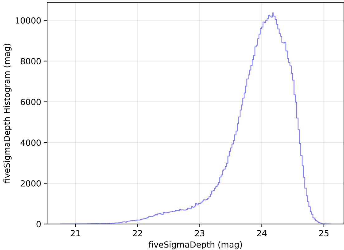
too_elab_heavy_r128_d2_gz_v3.4_10yrs All sky r band: fiveSigmaDepth Histogram
