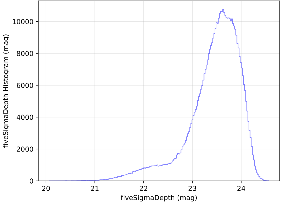
too_elab_heavy_r128_d2_gz_v3.4_10yrs All sky i band: fiveSigmaDepth Histogram
