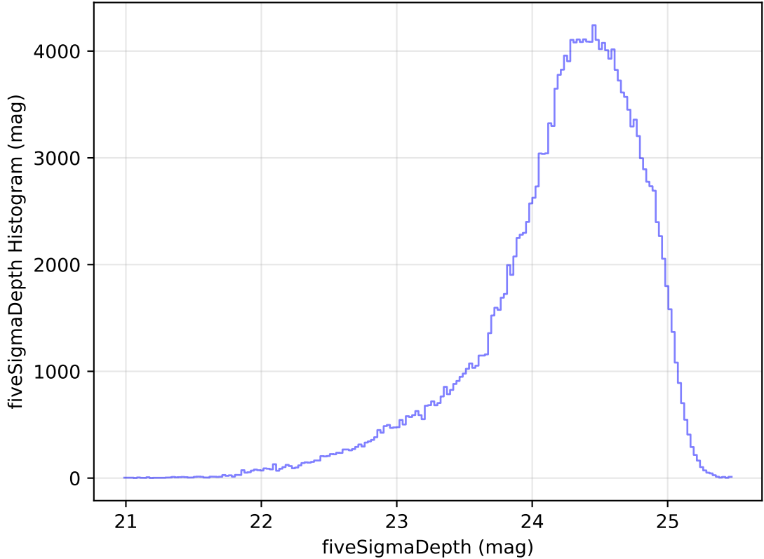
too_elab_heavy_r128_d2_gz_v3.4_10yrs All sky g band: fiveSigmaDepth Histogram
