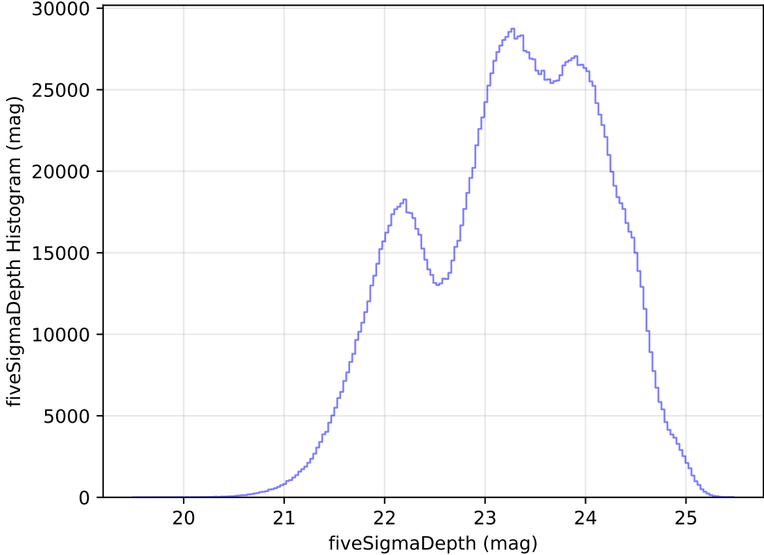
too_elab_heavy_r128_d2_gz_v3.4_10yrs All sky all bands: fiveSigmaDepth Histogram
