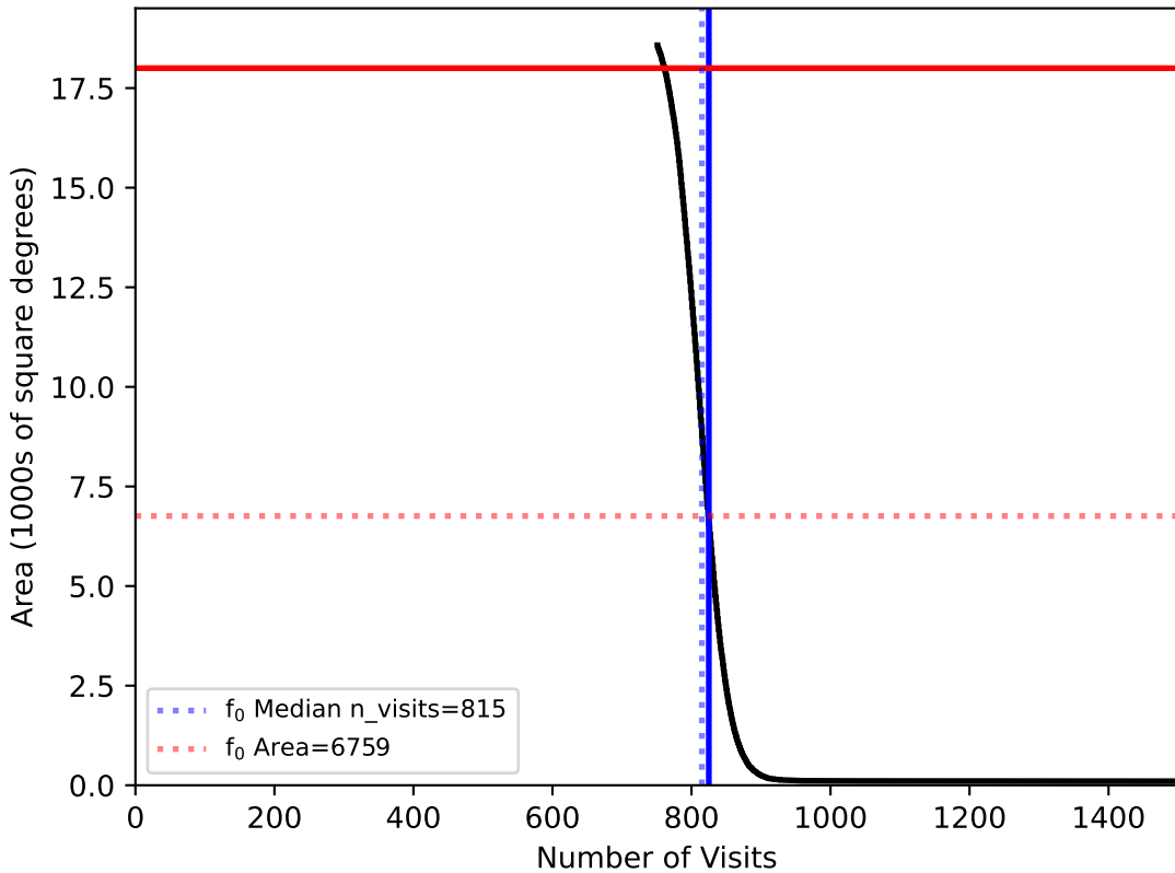
too_elab_heavy_r128_d2_gz_v3.4_10yrs WFD: fO
