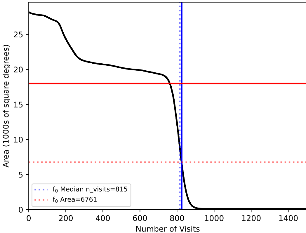
too_elab_heavy_r128_d2_gz_v3.4_10yrs All sky: f 0
