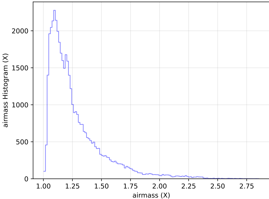
too_elab_heavy_r128_d2_gz_v3.4_10yrs Yr 1 z band: airmass Histogram
