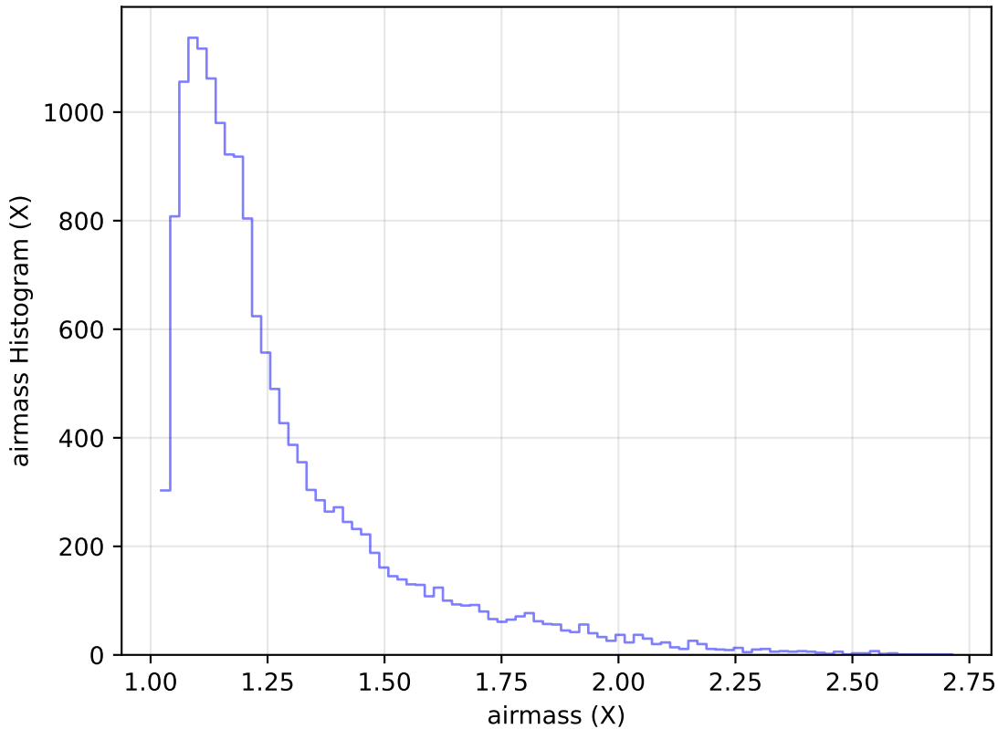
too_elab_heavy_r128_d2_gz_v3.4_10yrs Yr 1 u band: airmass Histogram
