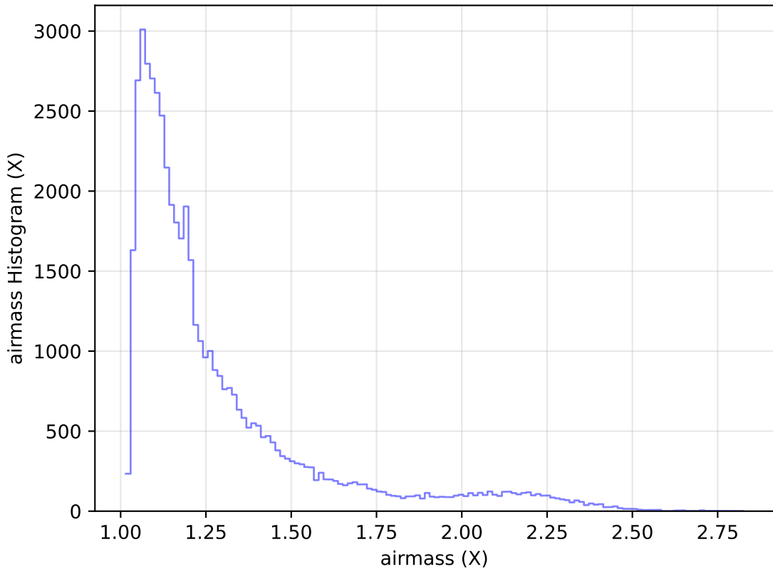
too_elab_heavy_r128_d2_gz_v3.4_10yrs Yr 1 r band: airmass Histogram
