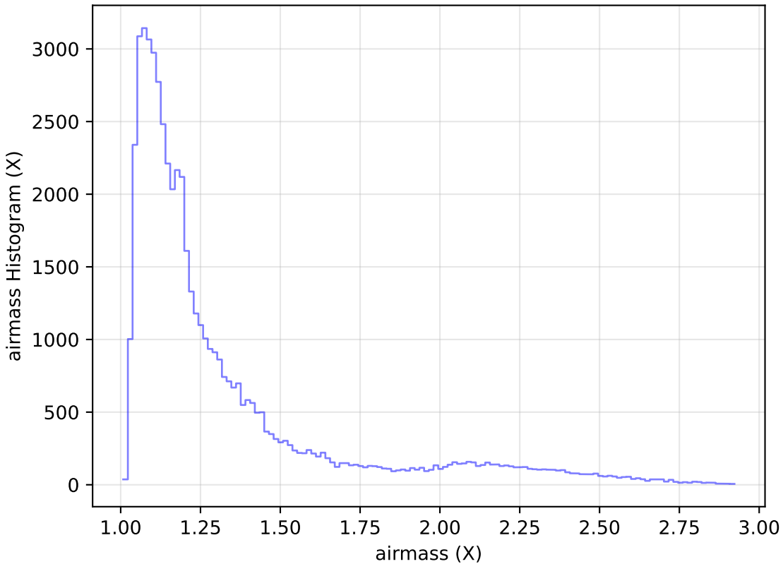
too_elab_heavy_r128_d2_gz_v3.4_10yrs Yr 1 i band: airmass Histogram
