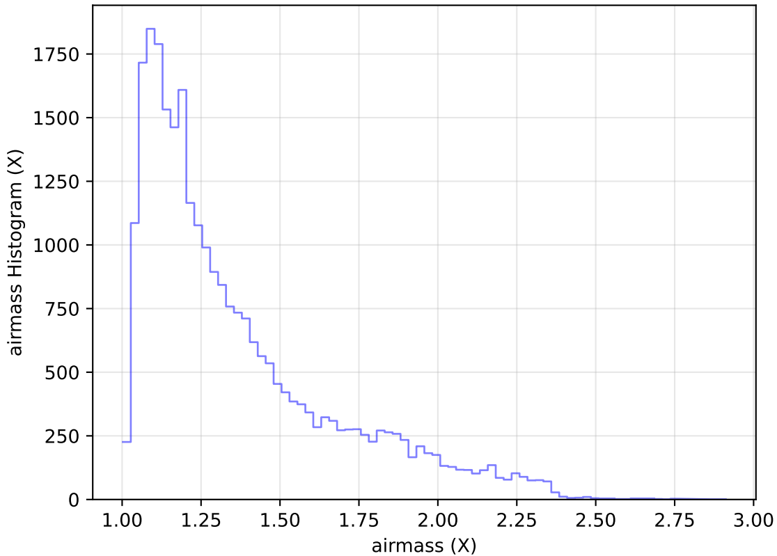
too_elab_heavy_r128_d2_gz_v3.4_10yrs Yr 1 g band: airmass Histogram
