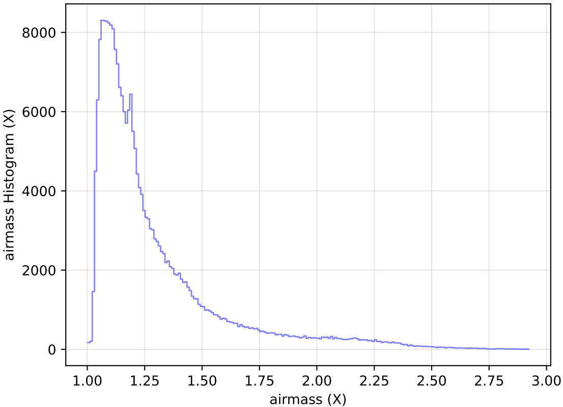
too_elab_heavy_r128_d2_gz_v3.4_10yrs Yr 1 all bands: airmass Histogram
