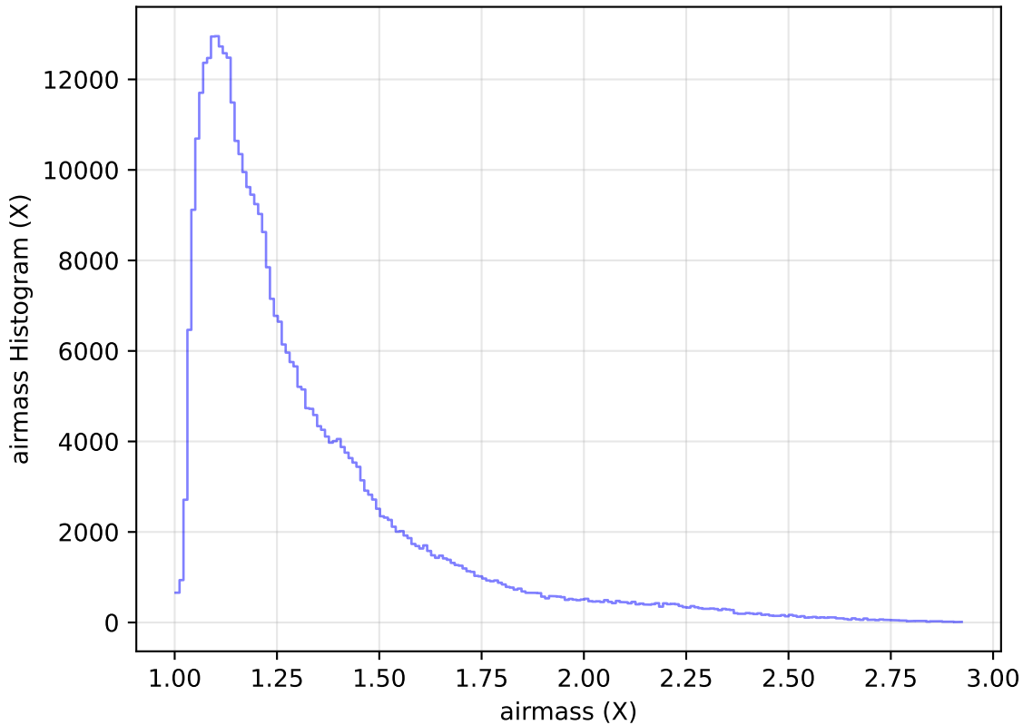
too_elab_heavy_r128_d2_gz_v3.4_10yrs WFD z band: airmass Histogram
