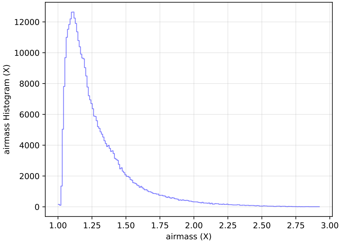
too_elab_heavy_r128_d2_gz_v3.4_10yrs WFD y band: airmass Histogram
