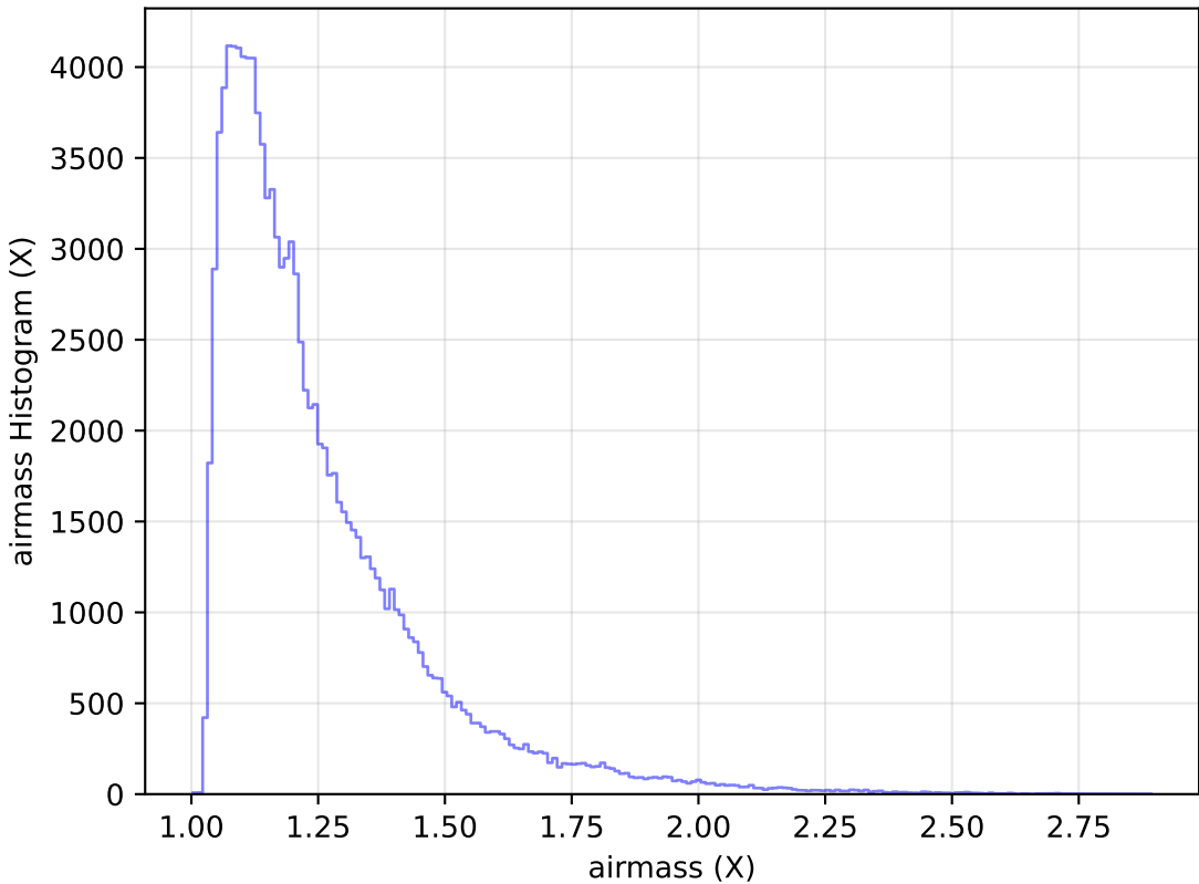
too_elab_heavy_r128_d2_gz_v3.4_10yrs WFD u band: airmass Histogram
