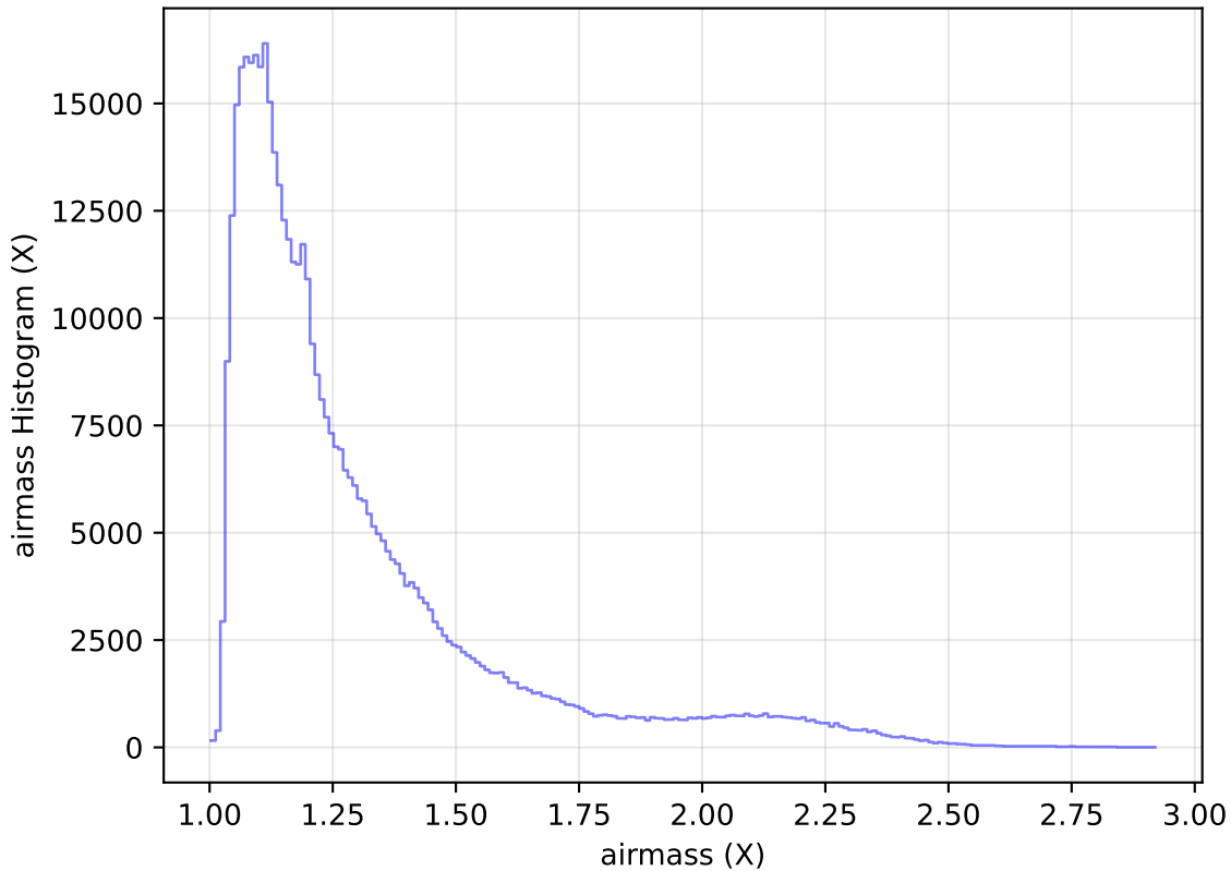
too_elab_heavy_r128_d2_gz_v3.4_10yrs WFD r band: airmass Histogram
