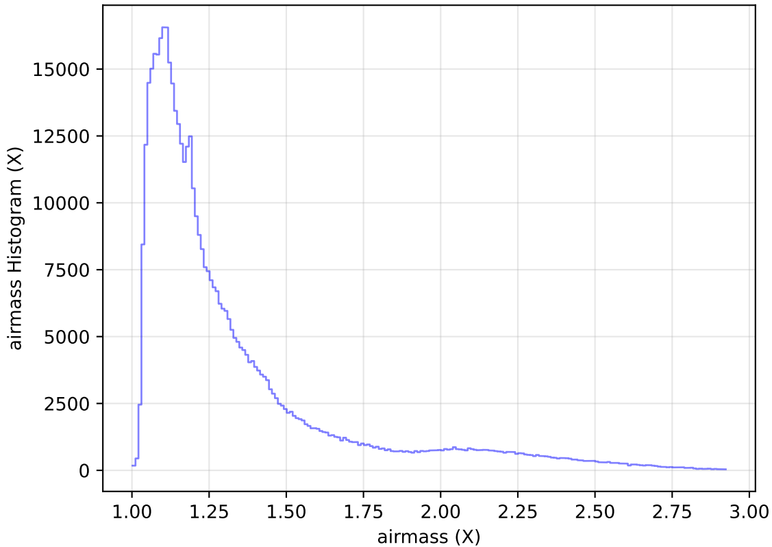
too_elab_heavy_r128_d2_gz_v3.4_10yrs WFD i band: airmass Histogram
