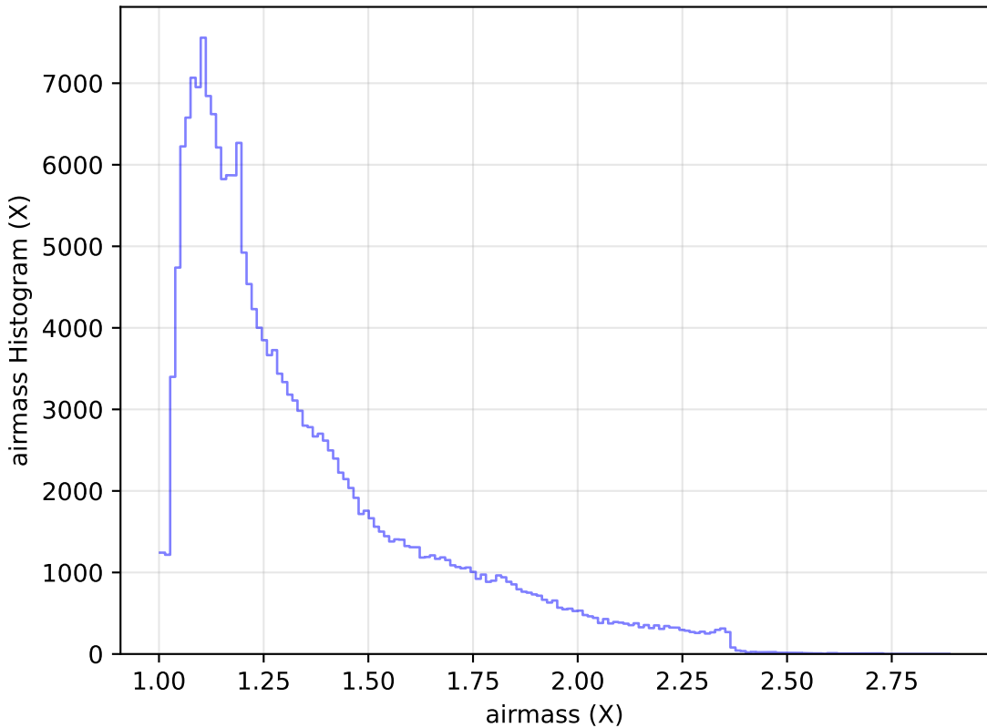
too_elab_heavy_r128_d2_gz_v3.4_10yrs WFD g band: airmass Histogram
