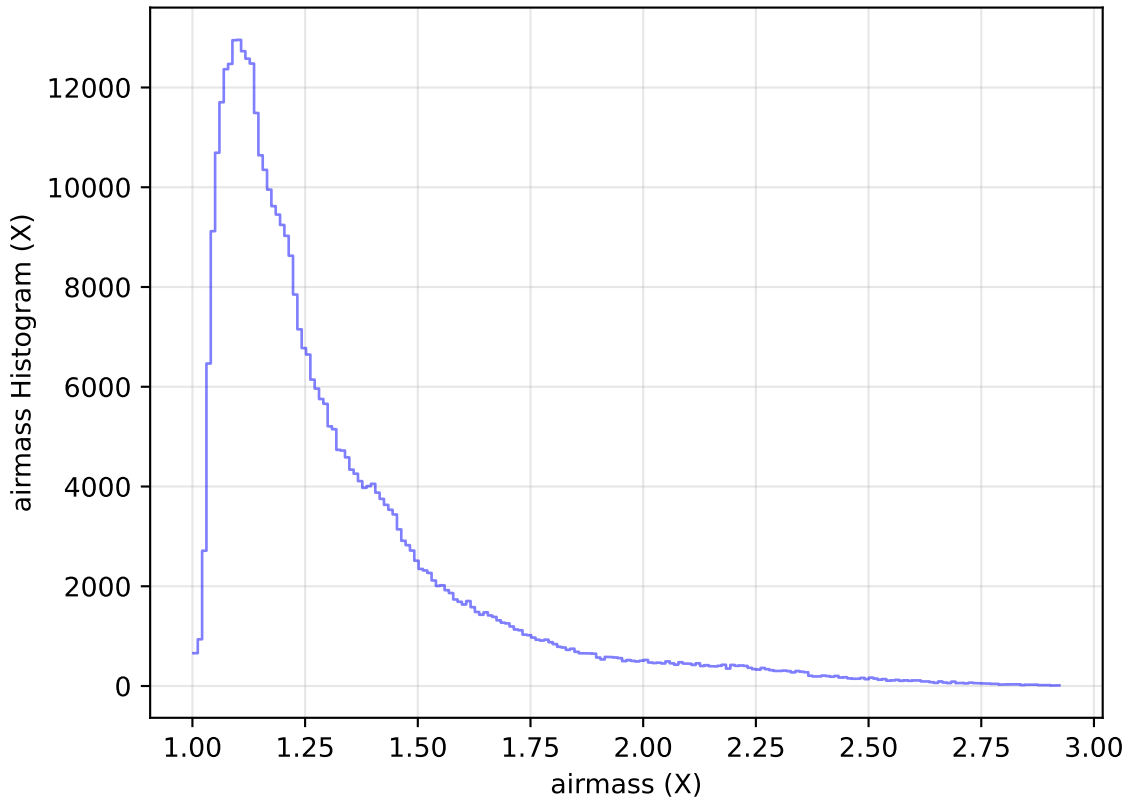
too_elab_heavy_r128_d2_gz_v3.4_10yrs All sky z band: airmass Histogram
