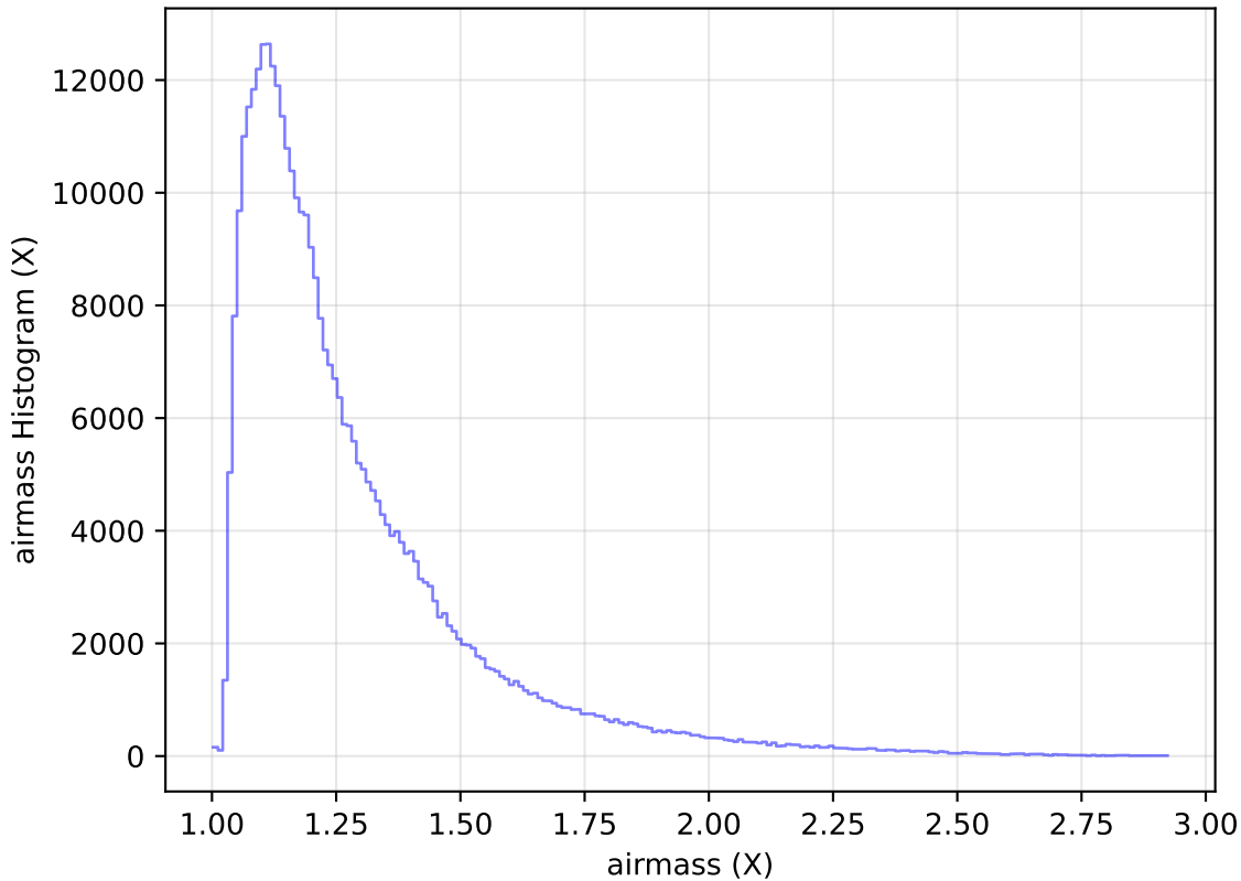
too_elab_heavy_r128_d2_gz_v3.4_10yrs All sky y band: airmass Histogram
