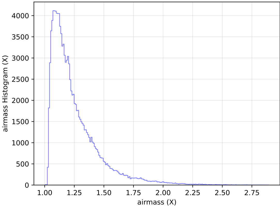
too_elab_heavy_r128_d2_gz_v3.4_10yrs All sky u band: airmass Histogram
