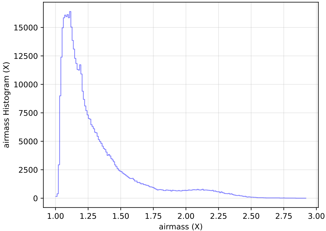
too_elab_heavy_r128_d2_gz_v3.4_10yrs All sky r band: airmass Histogram
