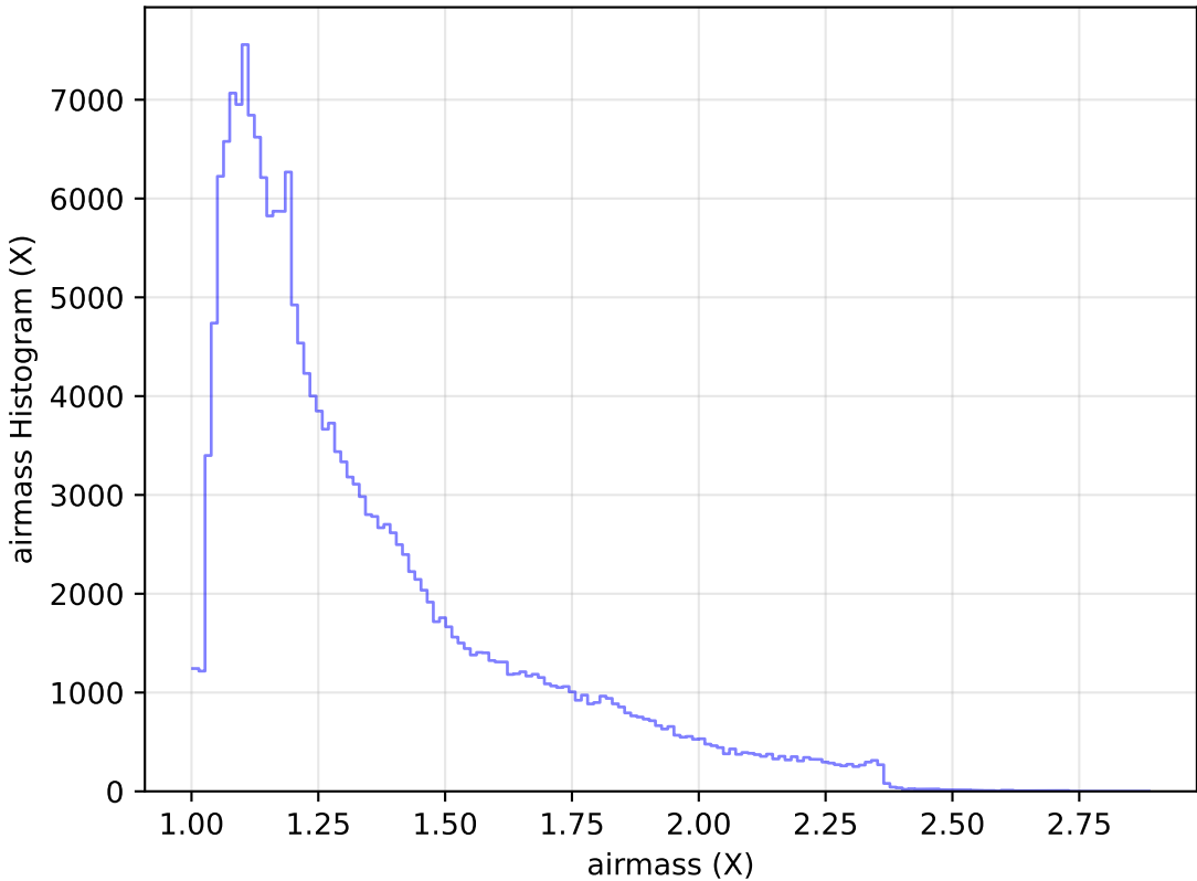
too_elab_heavy_r128_d2_gz_v3.4_10yrs All sky g band: airmass Histogram
