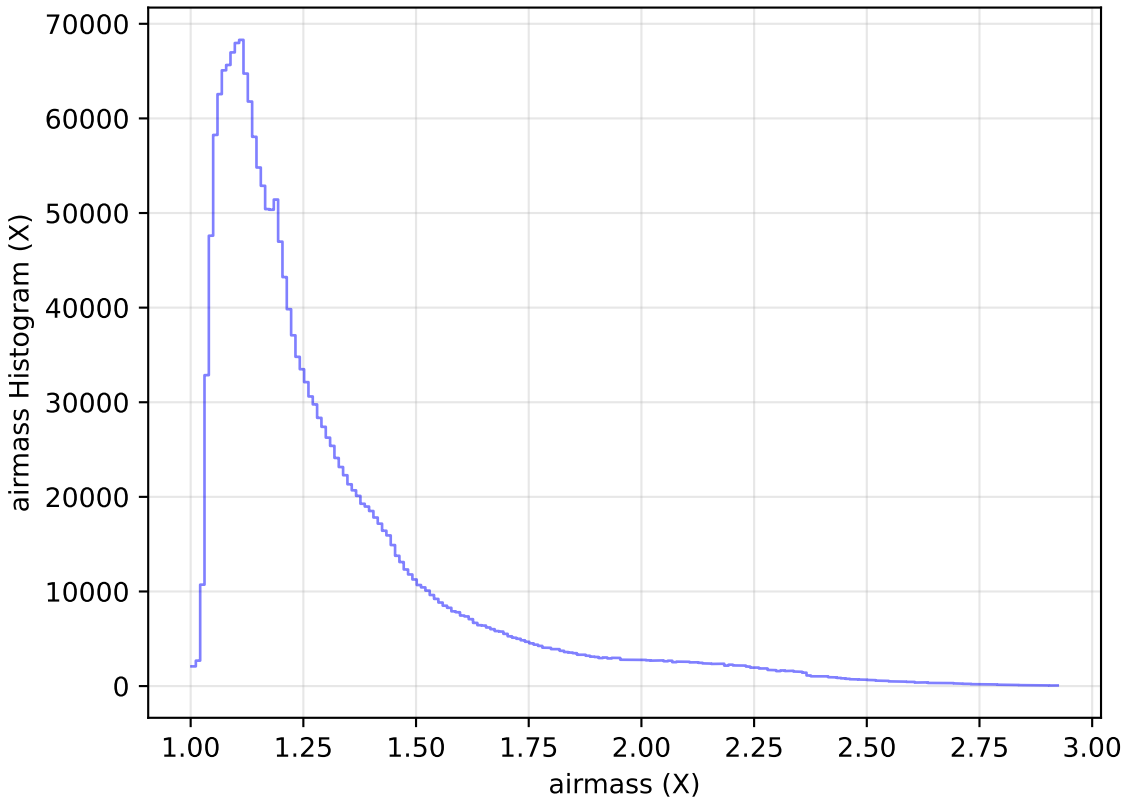
too_elab_heavy_r128_d2_gz_v3.4_10yrs All sky all bands: airmass Histogram
