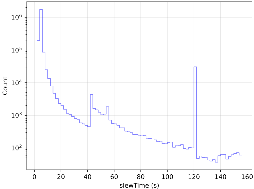
too_elab_heavy_r128_d2_gz_v3.4_10yrs All visits: Slew Time Histogram
