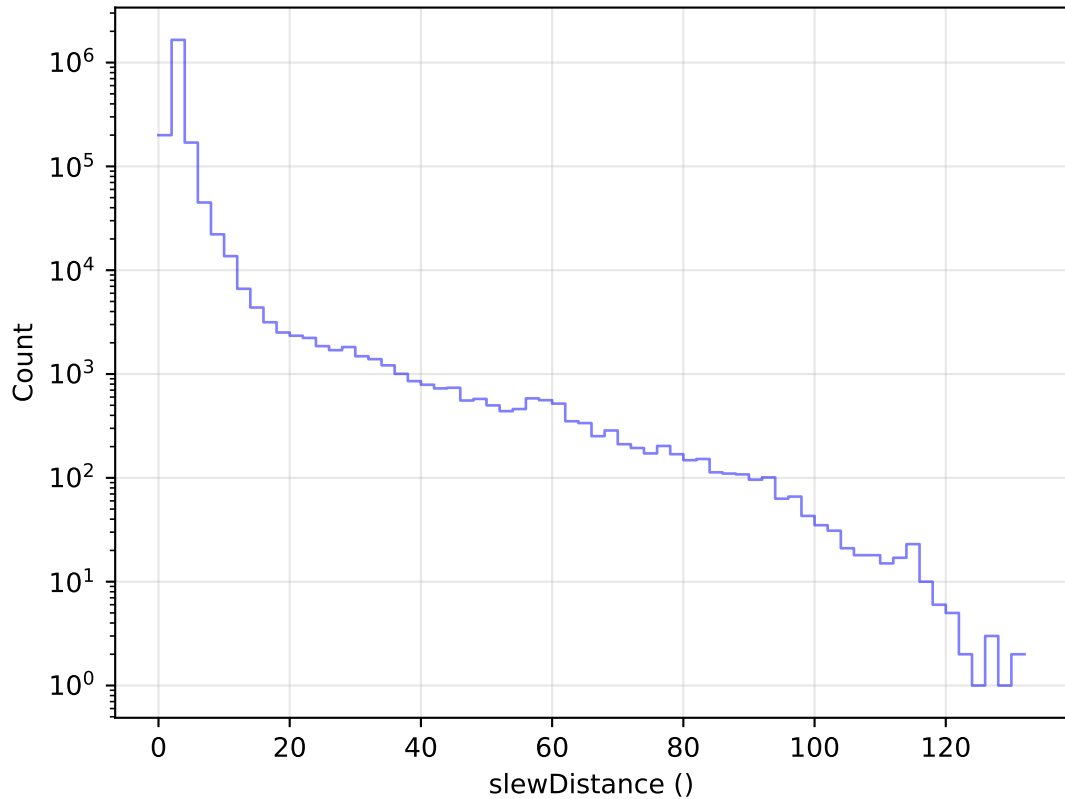
too_elab_heavy_r128_d2_gz_v3.4_10yrs All visits: Slew Distance Histogram
