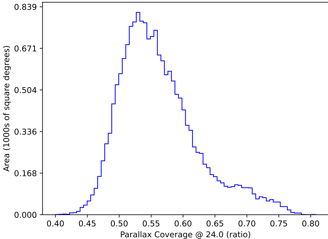
too_elab_heavy_r128_d2_gz_v3.4_10yrs WFD: Parallax Coverage @ 24.0
