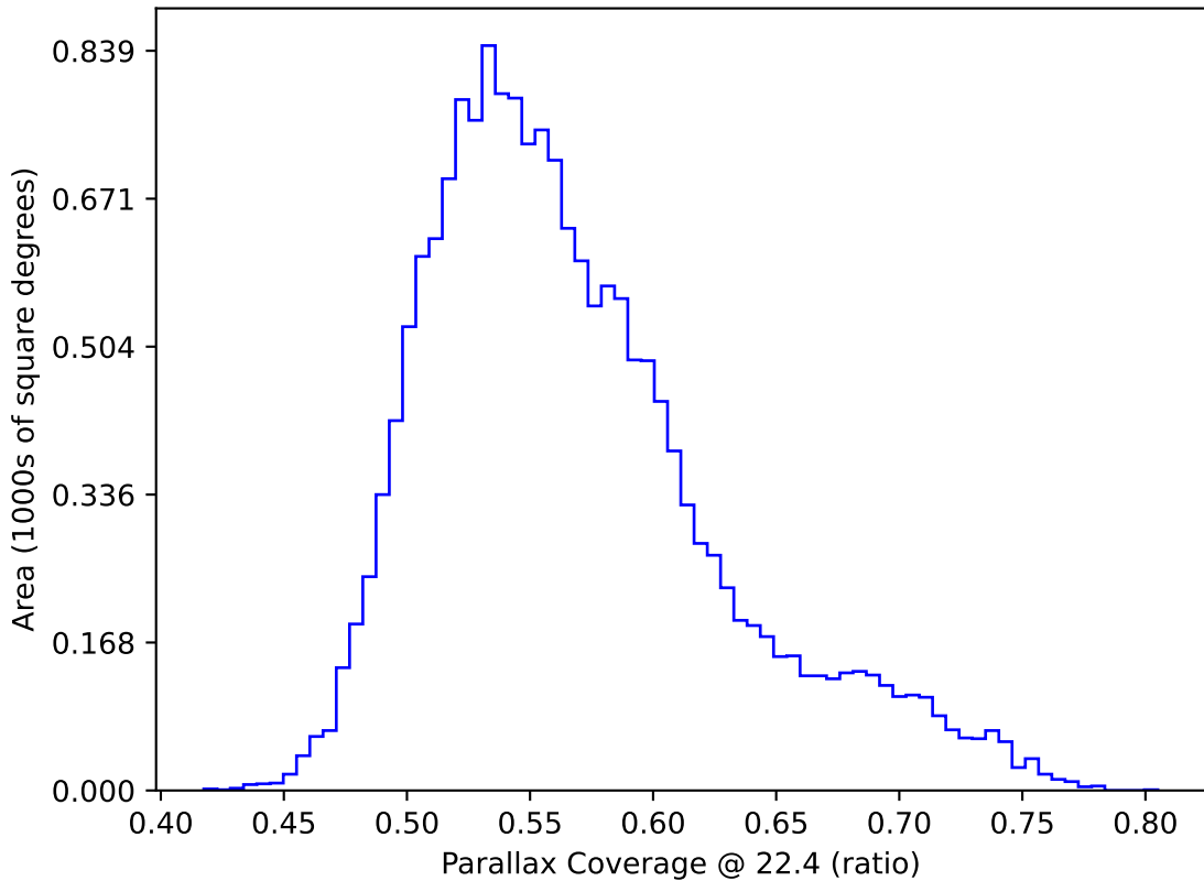
too_elab_heavy_r128_d2_gz_v3.4_10yrs WFD: Parallax Coverage @ 22.4
