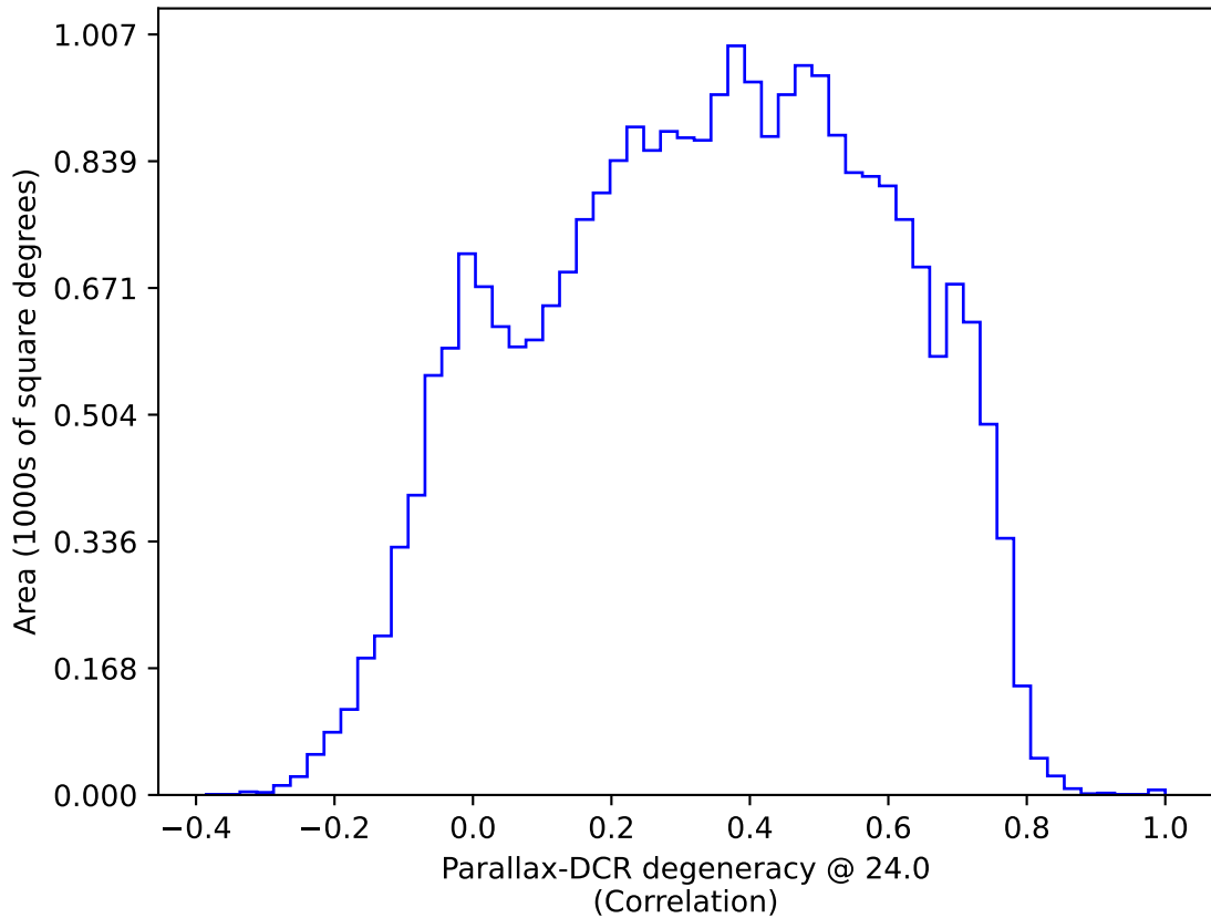
too_elab_heavy_r128_d2_gz_v3.4_10yrs All sky: Parallax-DCR degeneracy @ 24.0
