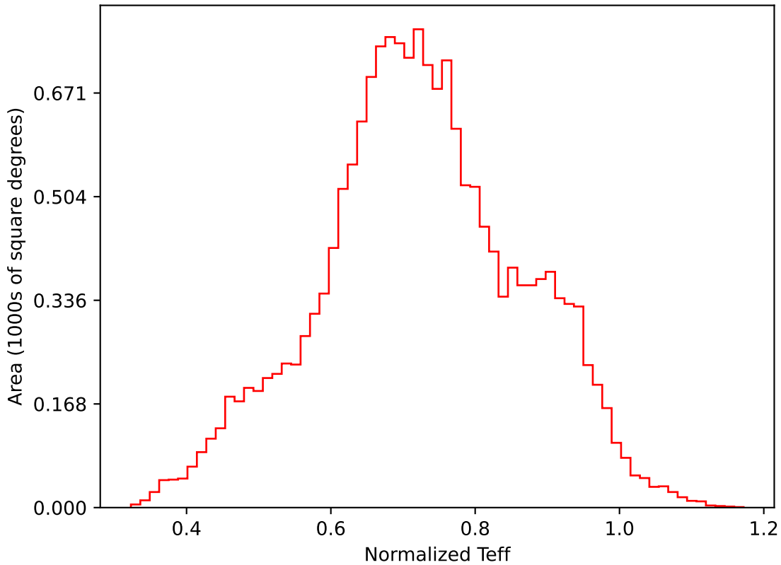
too_elab_heavy_r128_d2_gz_v3.4_10yrs WFD i band: Normalized Teff
