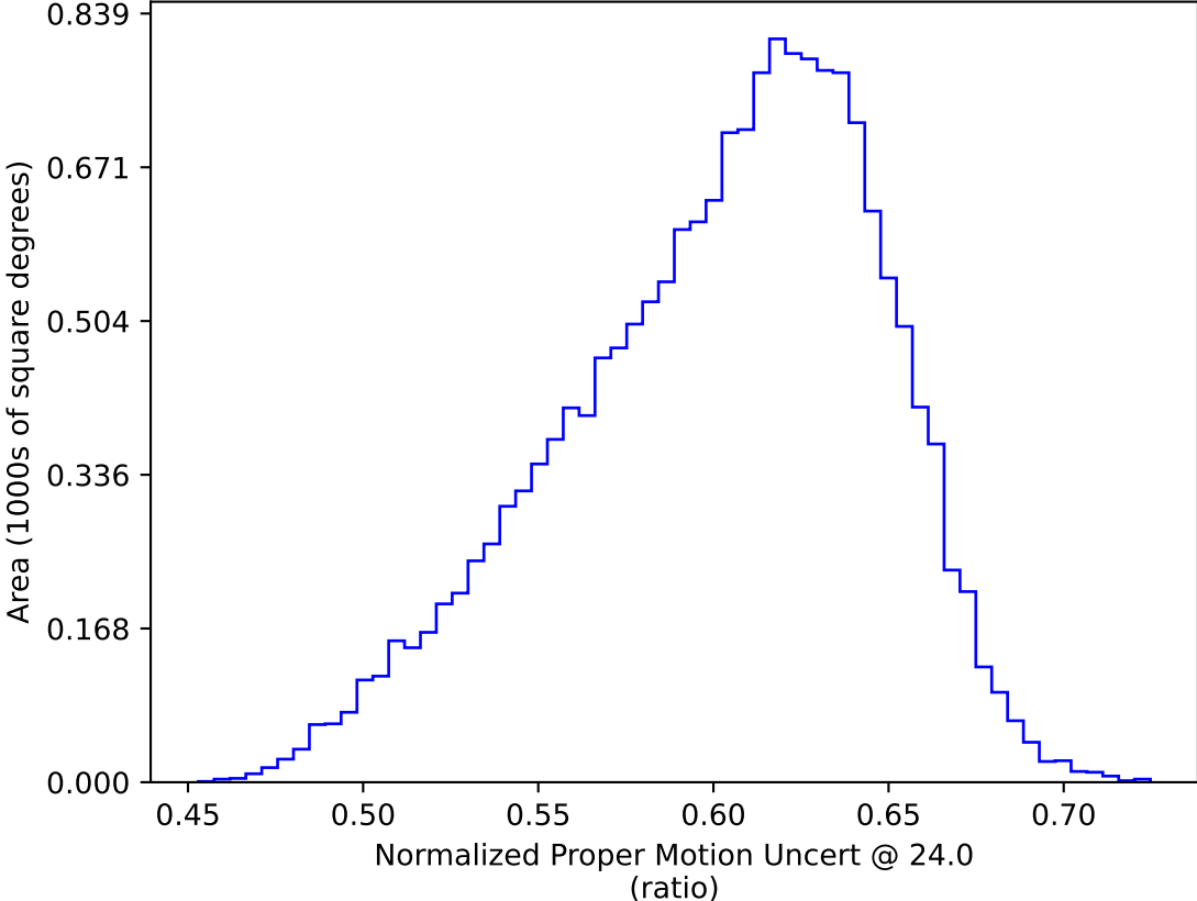
too_elab_heavy_r128_d2_gz_v3.4_10yrs WFD: Normalized Proper Motion Uncert @ 24.0
