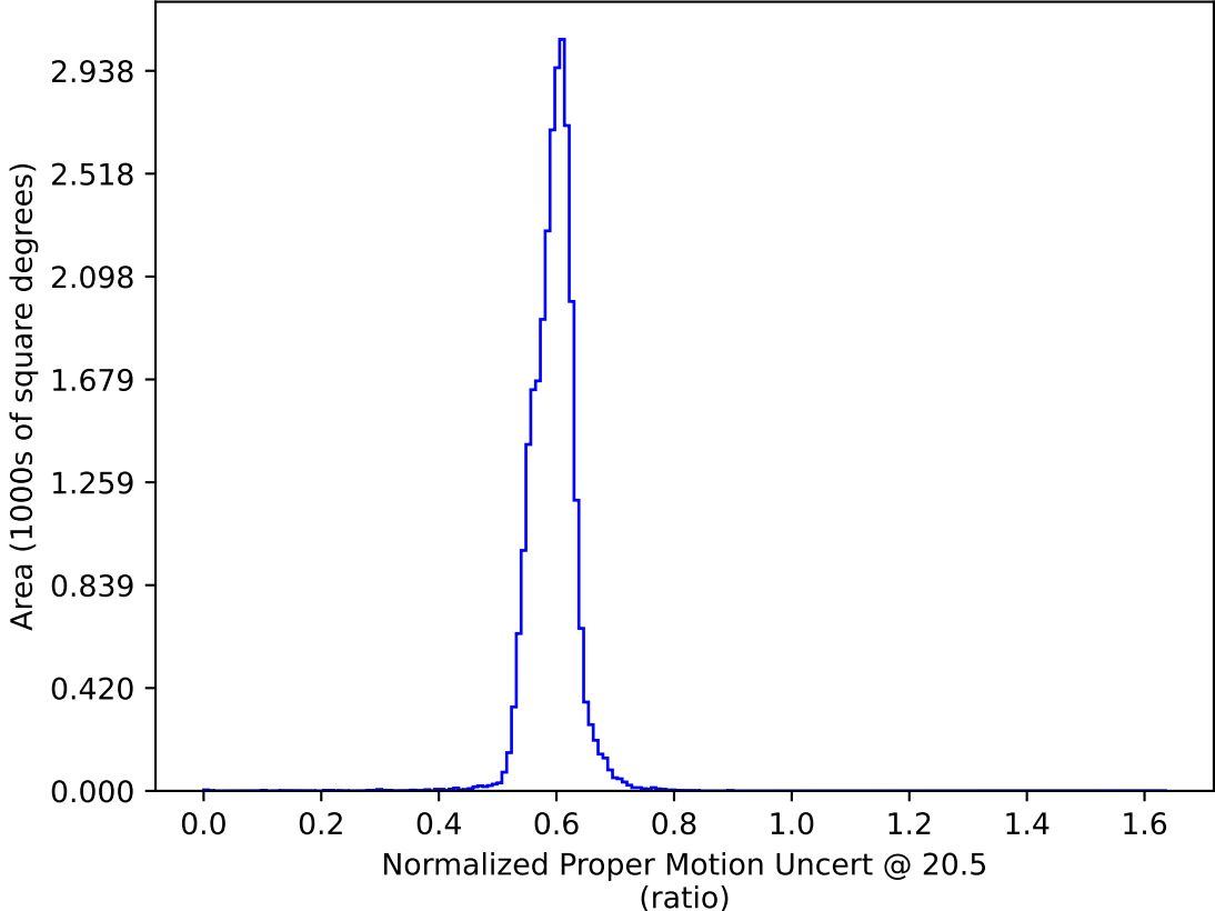
too_elab_heavy_r128_d2_gz_v3.4_10yrs All sky: Normalized Proper Motion Uncert @ 20.5
