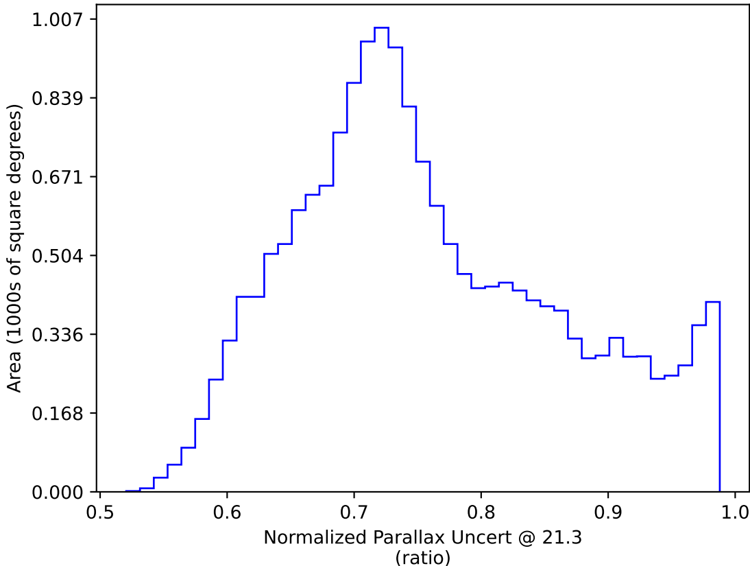
too_elab_heavy_r128_d2_gz_v3.4_10yrs WFD y band only: Normalized Parallax Uncert @ 21.3
