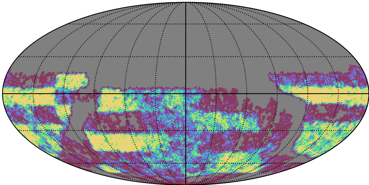
too_elab_heavy_r128_d2_gz_v3.4_10yrs Yr 3-4 u band: NVisits
