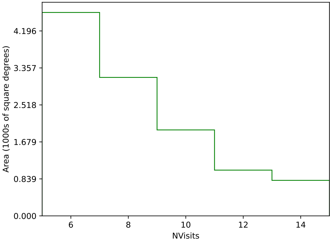
too_elab_heavy_r128_d2_gz_v3.4_10yrs Yr 3-4 g band: NVisits
