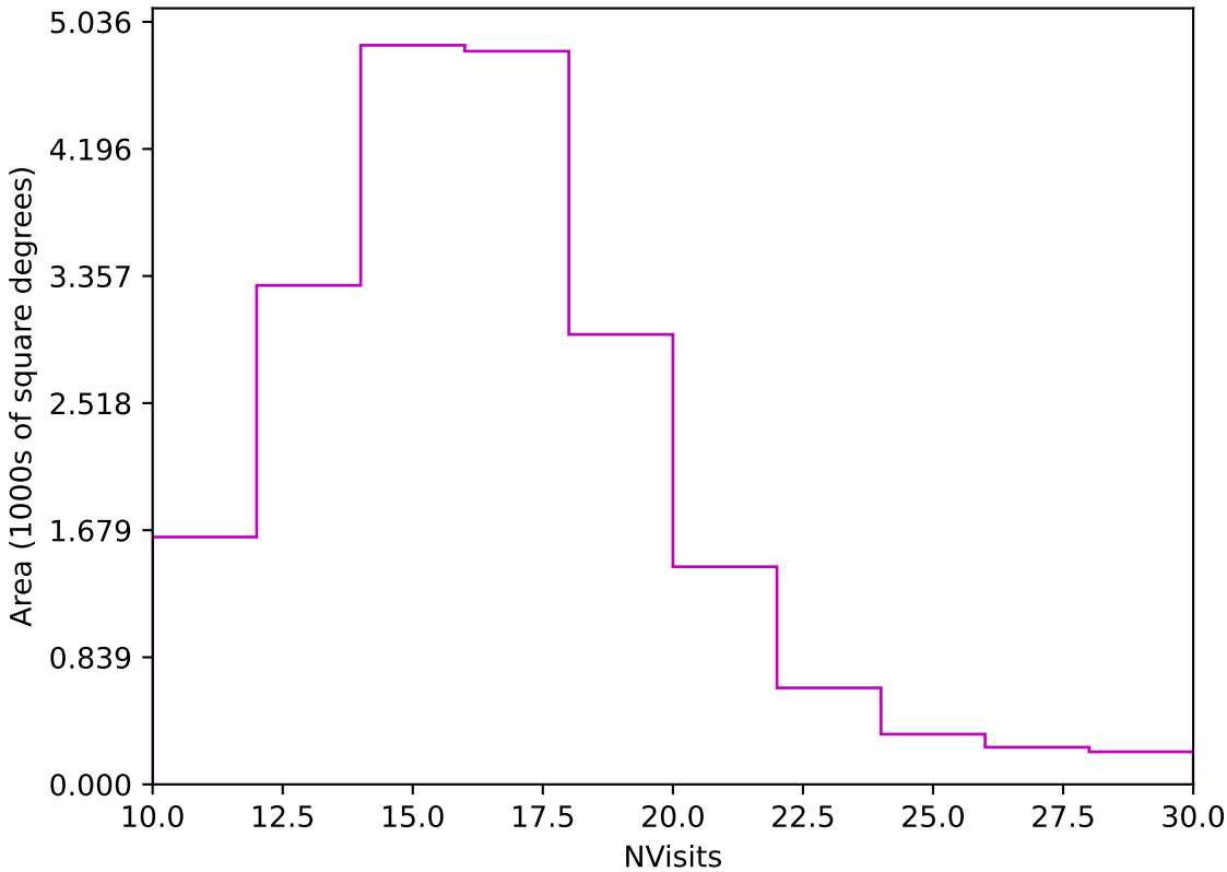
too_elab_heavy_r128_d2_gz_v3.4_10yrs Yr 1 z band: NVisits
