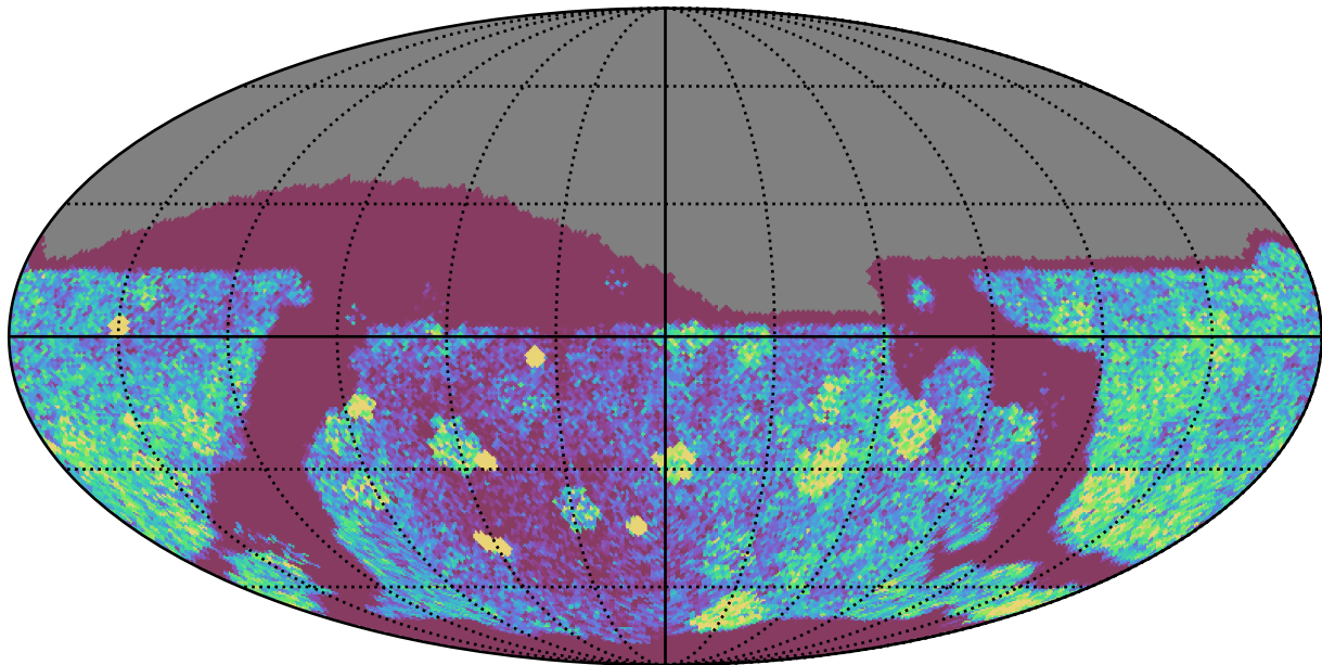
too_elab_heavy_r128_d2_gz_v3.4_10yrs Yr 1 all bands: NVisits
