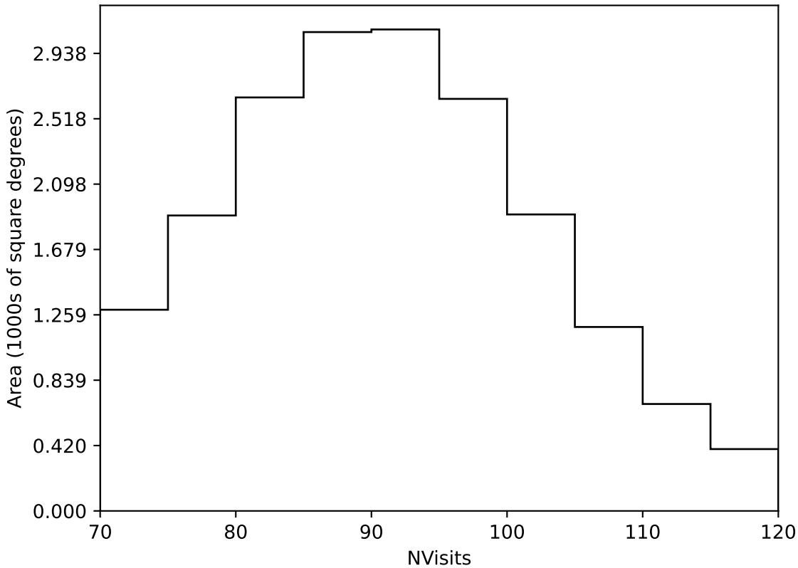
too_elab_heavy_r128_d2_gz_v3.4_10yrs Yr 1 all bands: NVisits
