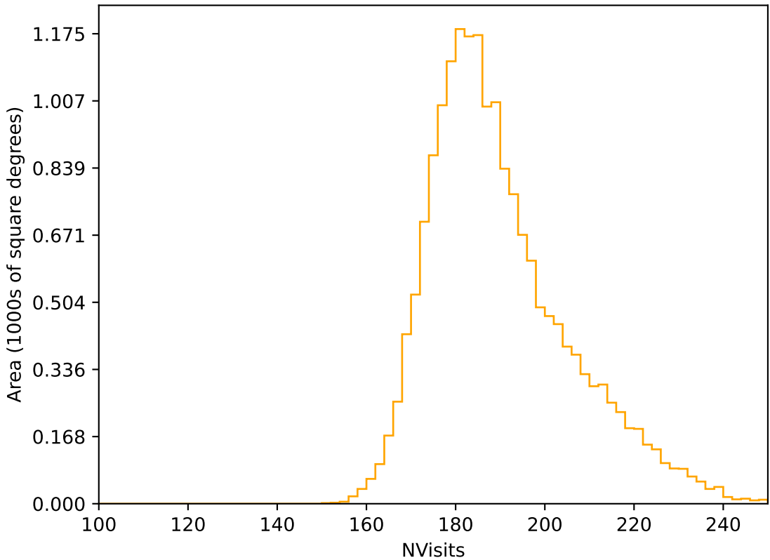
too_elab_heavy_r128_d2_gz_v3.4_10yrs WFD r band: NVisits
