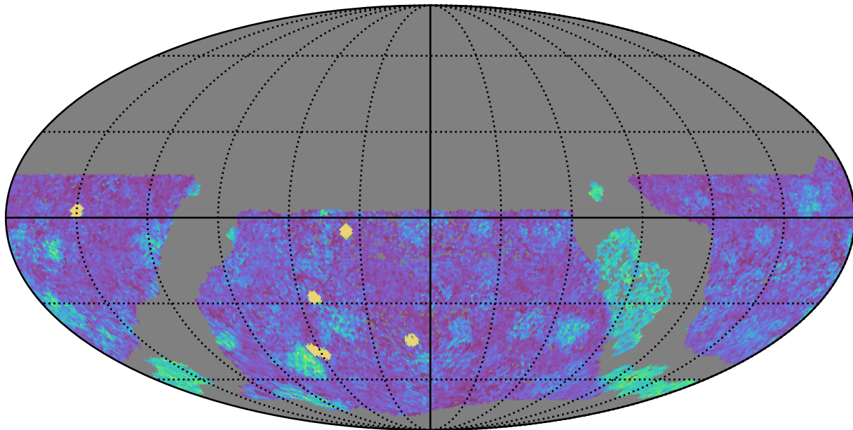
too_elab_heavy_r128_d2_gz_v3.4_10yrs WFD g band: NVisits
