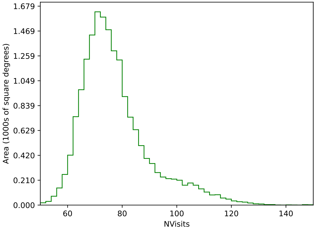
too_elab_heavy_r128_d2_gz_v3.4_10yrs WFD g band: NVisits
