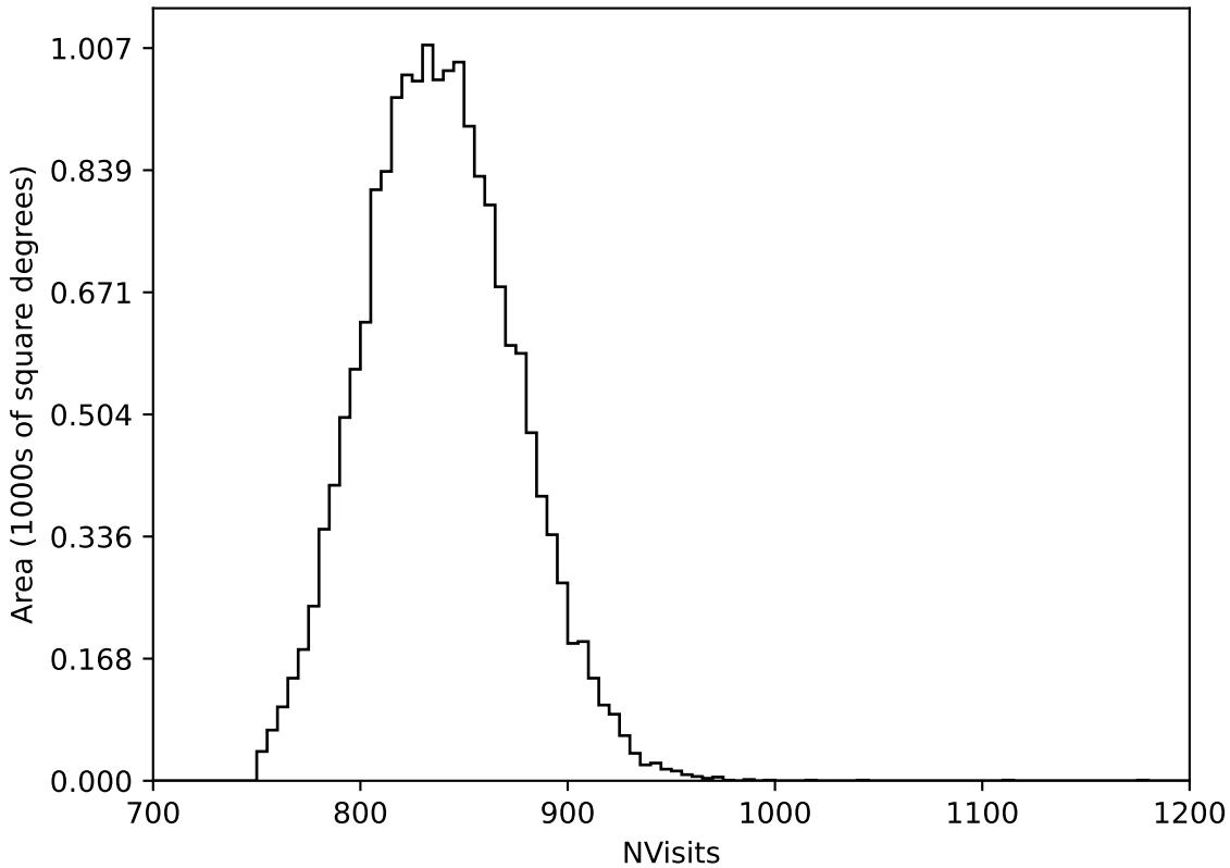
too_elab_heavy_r128_d2_gz_v3.4_10yrs WFD all bands: NVisits
