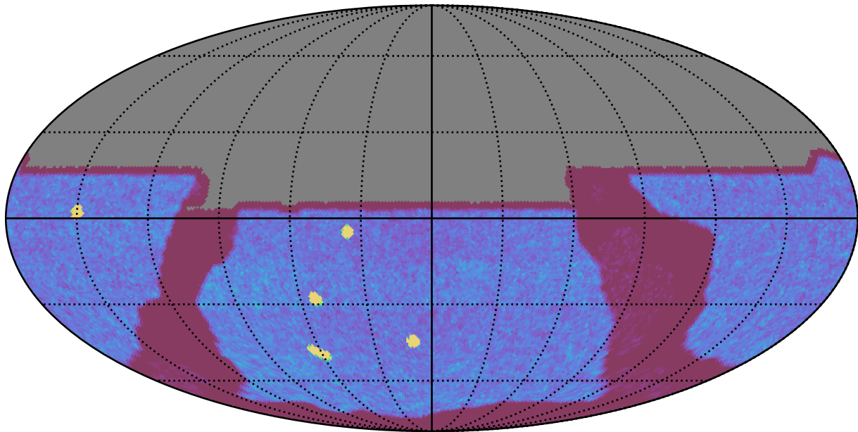
too_elab_heavy_r128_d2_gz_v3.4_10yrs All sky y band: NVisits
