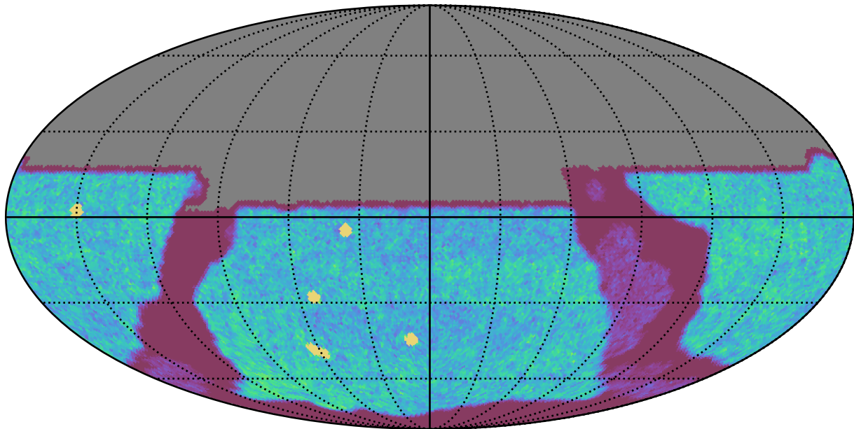
too_elab_heavy_r128_d2_gz_v3.4_10yrs All sky u band: NVisits
