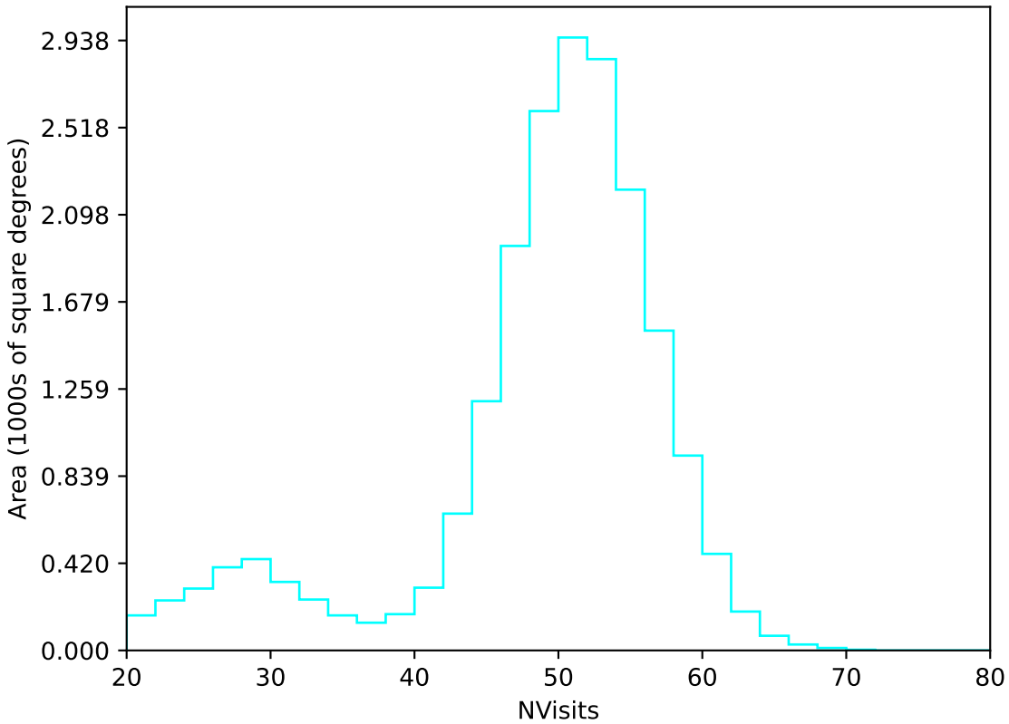
too_elab_heavy_r128_d2_gz_v3.4_10yrs All sky u band: NVisits
