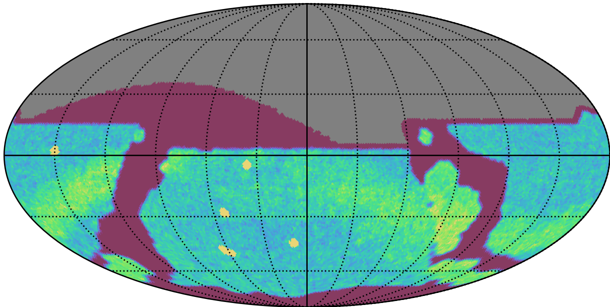
too_elab_heavy_r128_d2_gz_v3.4_10yrs All sky r band: NVisits
