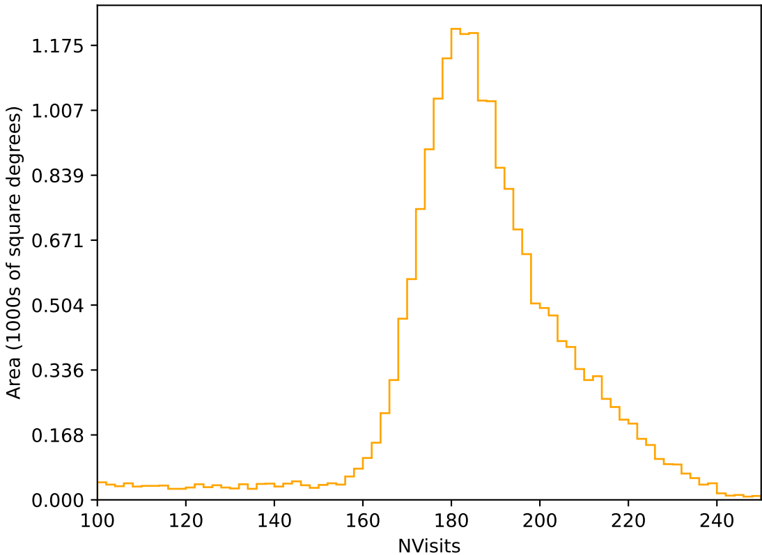
too_elab_heavy_r128_d2_gz_v3.4_10yrs All sky r band: NVisits
