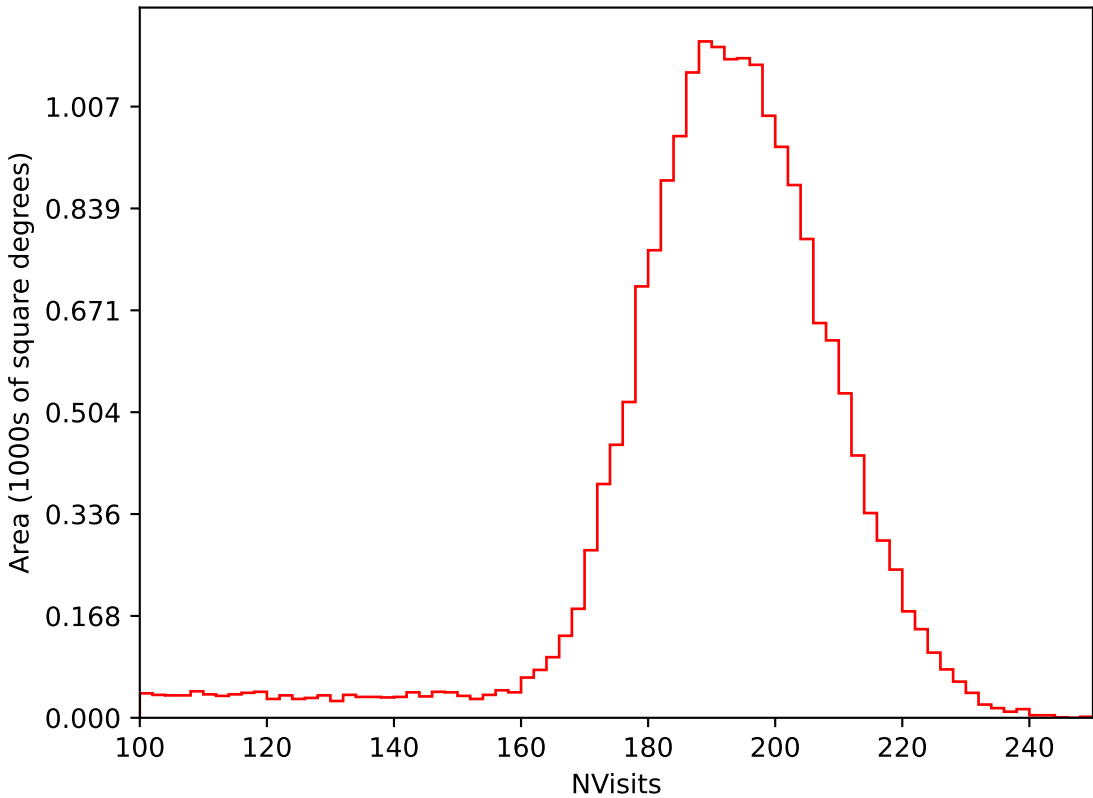
too_elab_heavy_r128_d2_gz_v3.4_10yrs All sky i band: NVisits
